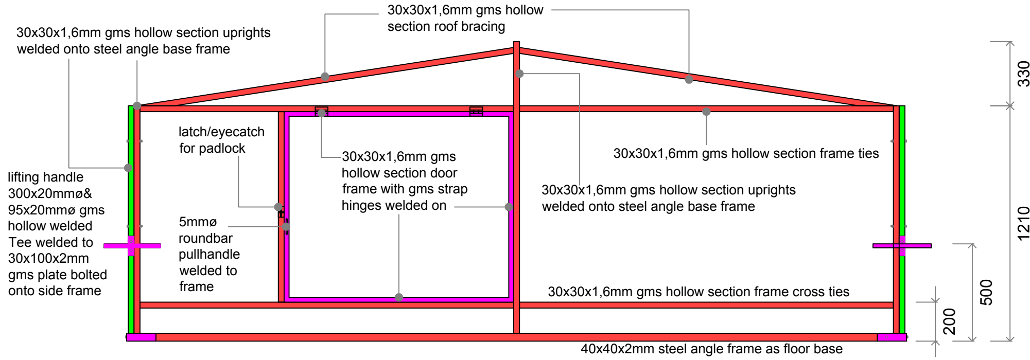
front view 1:20
