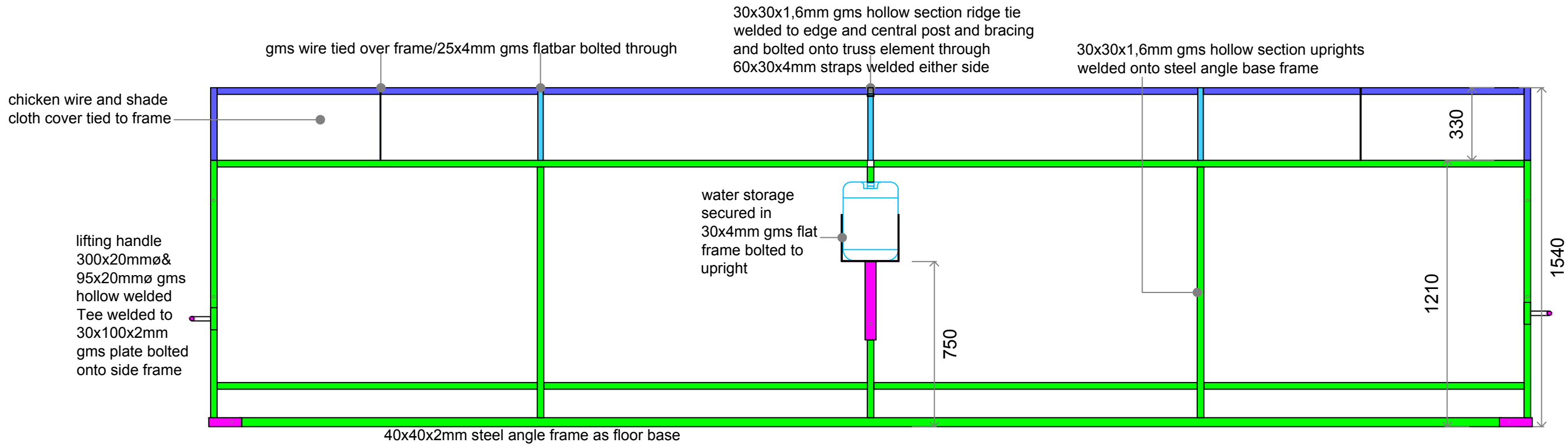
side view 1:20
